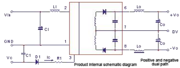
Recommended Circuit 1&2
