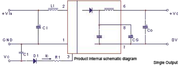
Recommended Circuit 1&2
